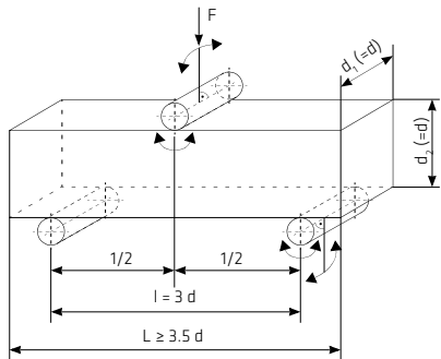
Figure 4.3.3.4: Central load transfer
