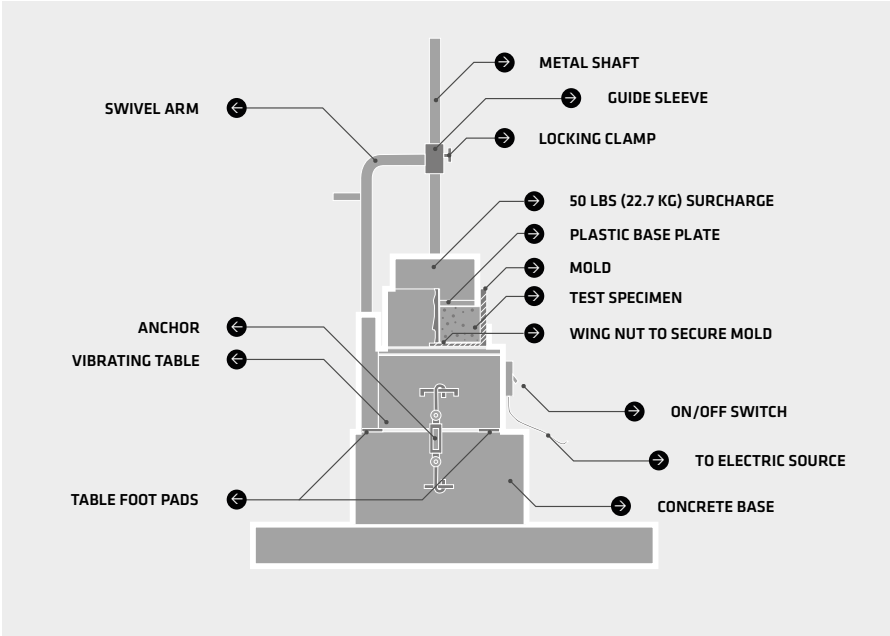
Figure 4.2.1.3: Vebe apparatus
