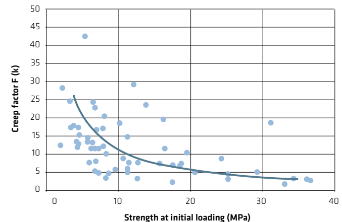
Figure 4.3.5.1: Creep factor vs. strength at initial loading (various mixes from several projects)
